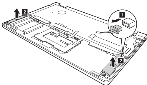
Figure 9. Removal steps of speakers
