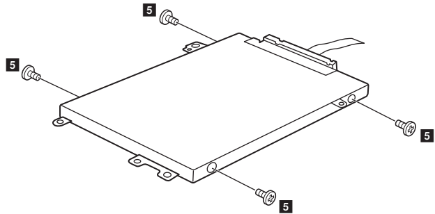
Figure 3. Removal steps of hard disk drive (continued) Remove four screws 5 and detach the metal frame from the hard disk drive.
